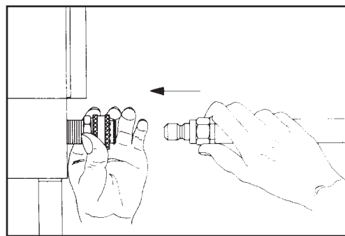
ILLUSTRATION #7 HIGH PRESSURE HOSE CONNECTION
