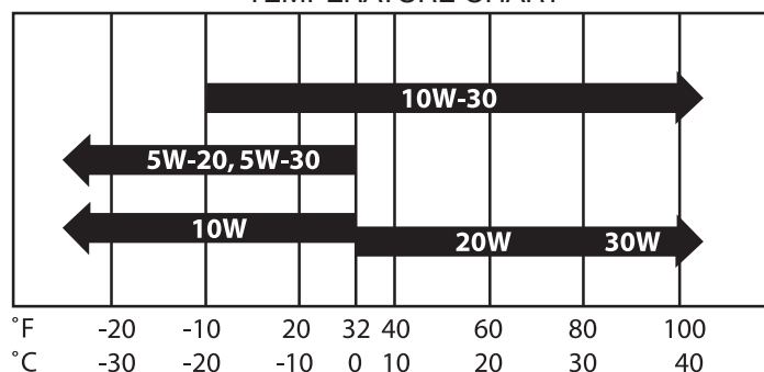
TEMPERATURE CHART
