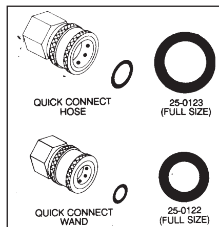
Illustration #16 Quick Couplers
