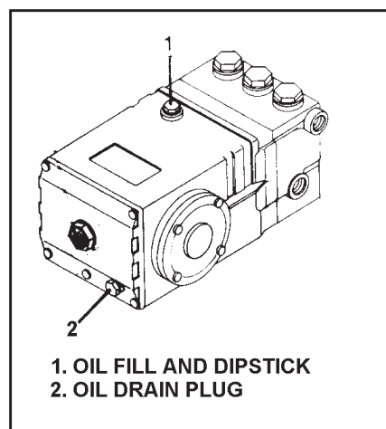
Illustration #17 Pump Oil Drain
