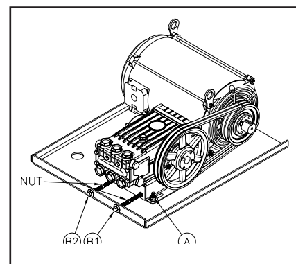
Illustration #18 Belt Tension Adjustment
