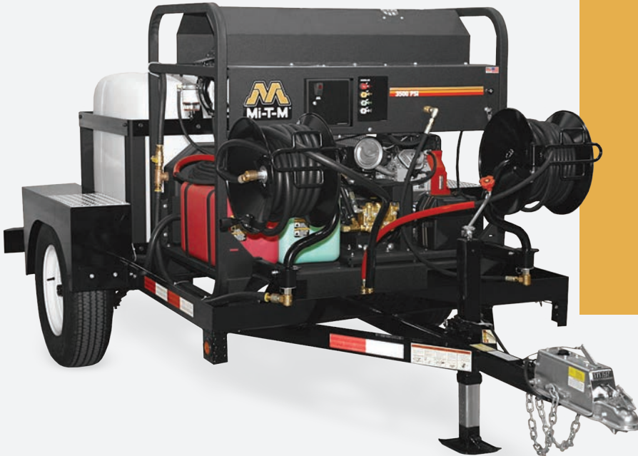
AW-9000-0005 single-axle trailer shown with HS-3505-1MGH hot water pressure washer, hose reels and industrial supply hose, 15-0006 (available as accessories)
