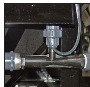
Mazzei® venturi air injection system sustains beneficial aerobic microbes while preventing bacteria from turning odorous and anaerobic
